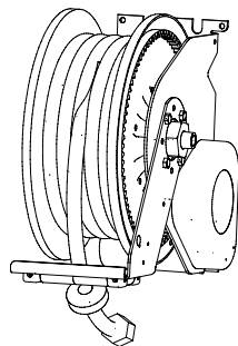
WALL MOUNT CONFIGURATION
