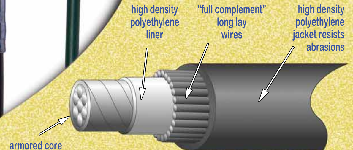
Throttle Cables
