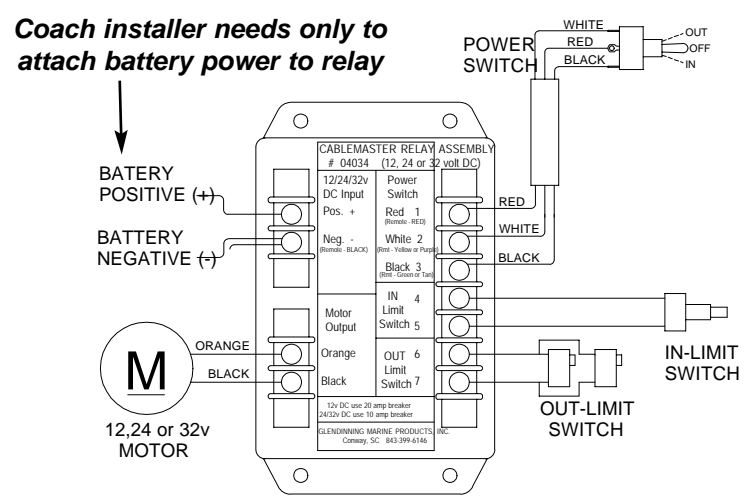
TYPICAL RVCM-7 RELAY ASSEMBLY WIRING
